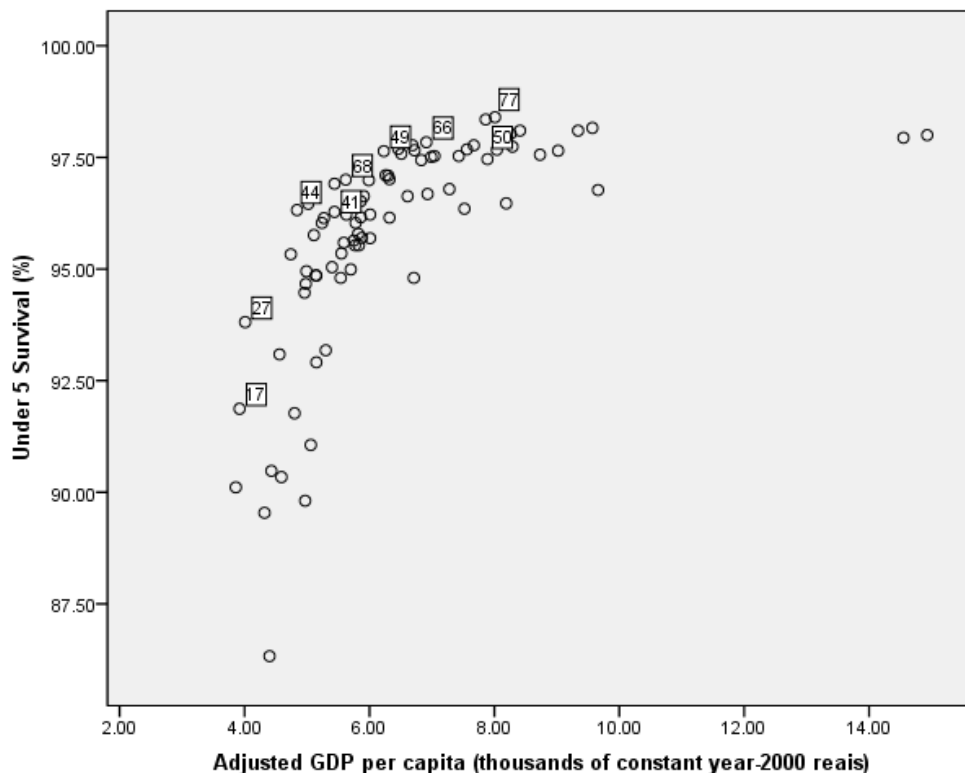
Figure 2: Sample Scatter-Plot with Frontier Observations
